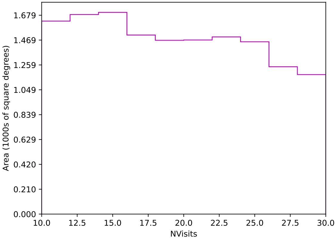
too_elab_2yr_r32_d2_ugrizy_v3.4_10yrs Yr 3-4 z band: NVisits
