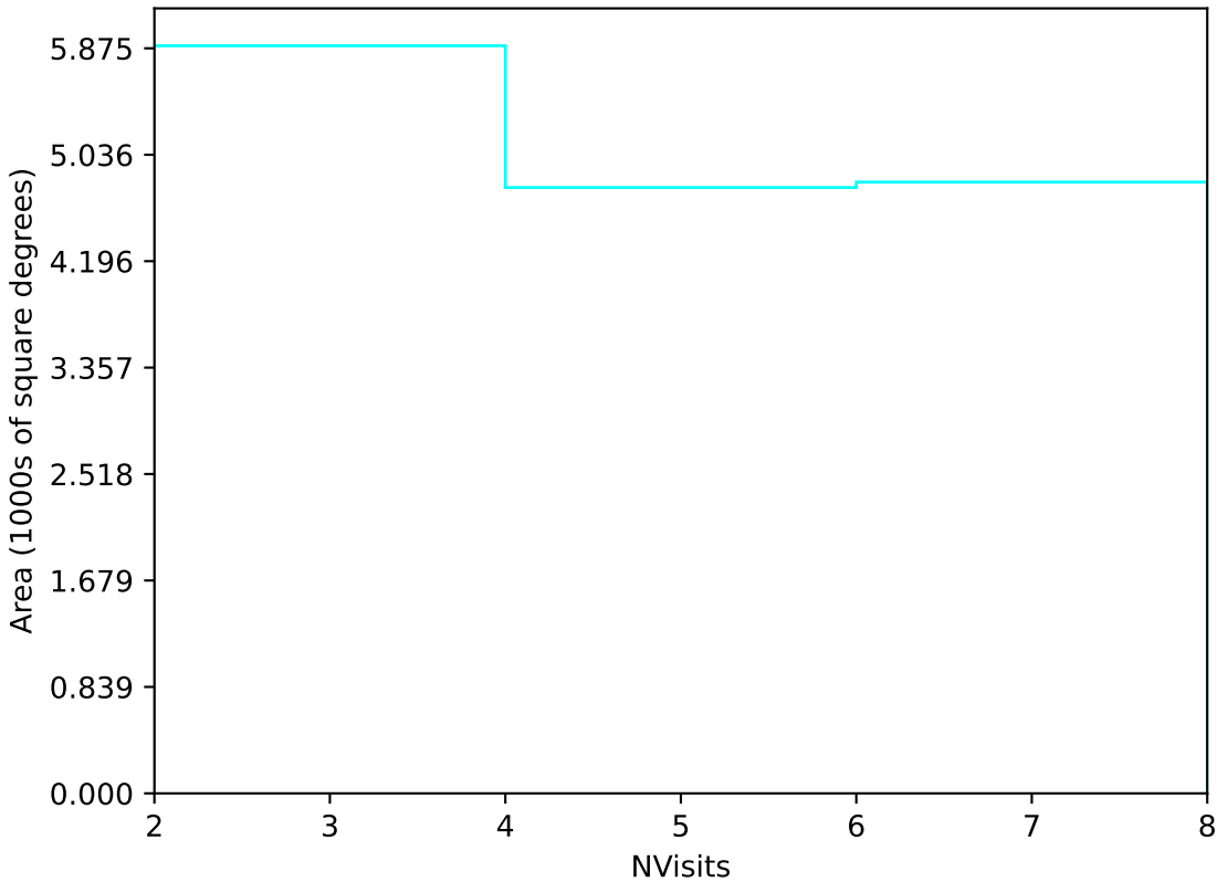
too_elab_2yr_r32_d2_ugrizy_v3.4_10yrs Yr 3-4 u band: NVisits
