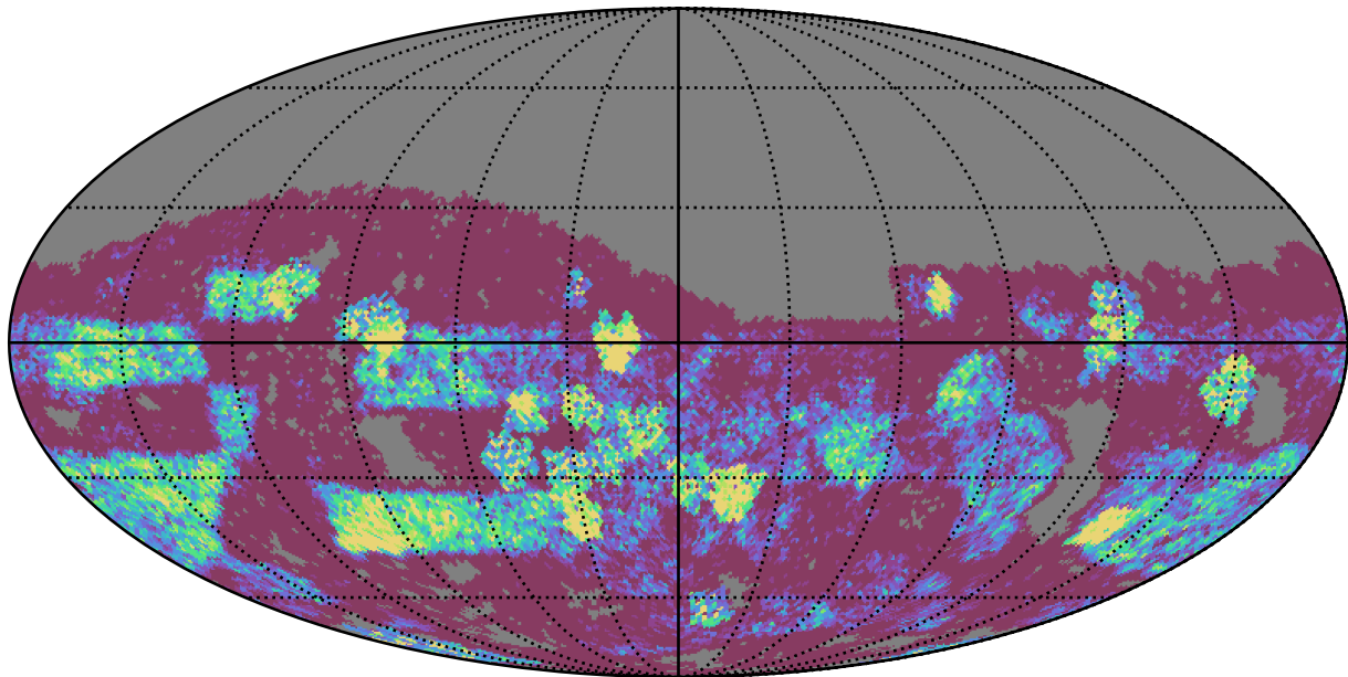
too_elab_2yr_r32_d2_ugrizy_v3.4_10yrs Yr 3-4 g band: NVisits
