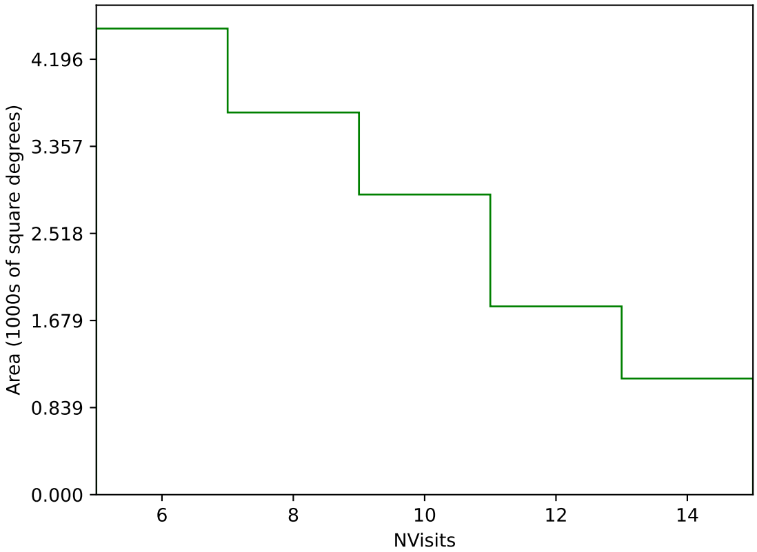
too_elab_2yr_r32_d2_ugrizy_v3.4_10yrs Yr 3-4 g band: NVisits
