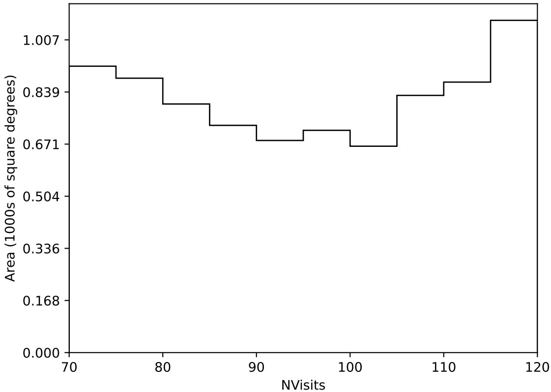
too_elab_2yr_r32_d2_ugrizy_v3.4_10yrs Yr 3-4 all bands: NVisits
