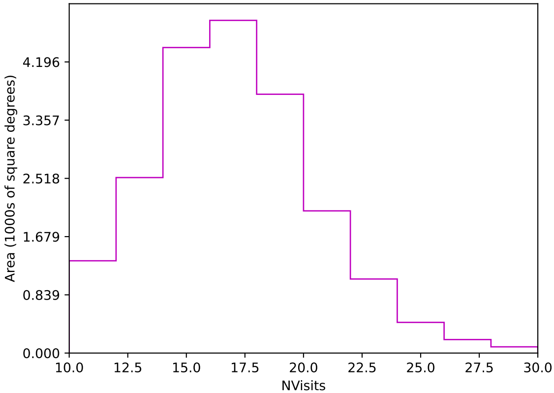
too_elab_2yr_r32_d2_ugrizy_v3.4_10yrs Yr 1 z band: NVisits
