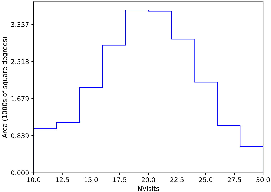
too_elab_2yr_r32_d2_ugrizy_v3.4_10yrs Yr 1 y band: NVisits
