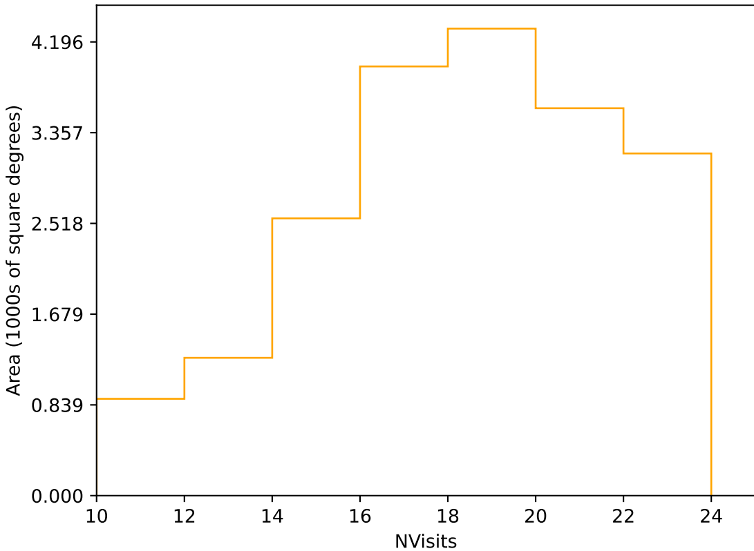
too_elab_2yr_r32_d2_ugrizy_v3.4_10yrs Yr 1 r band: NVisits
