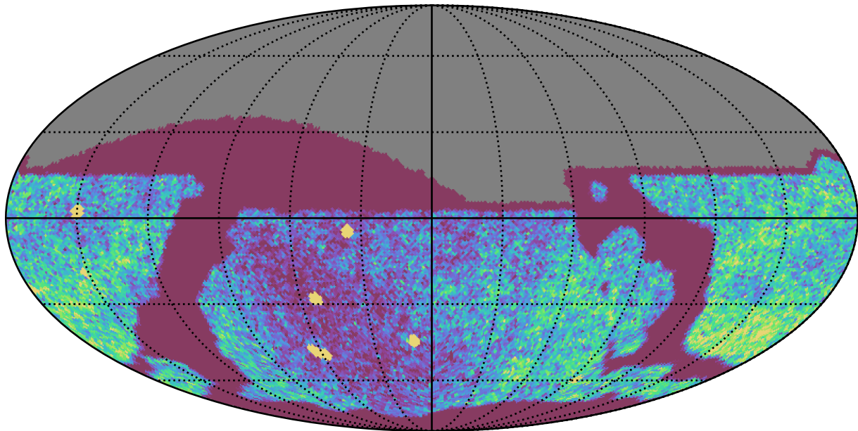
too_elab_2yr_r32_d2_ugrizy_v3.4_10yrs Yr 1 all bands: NVisits
