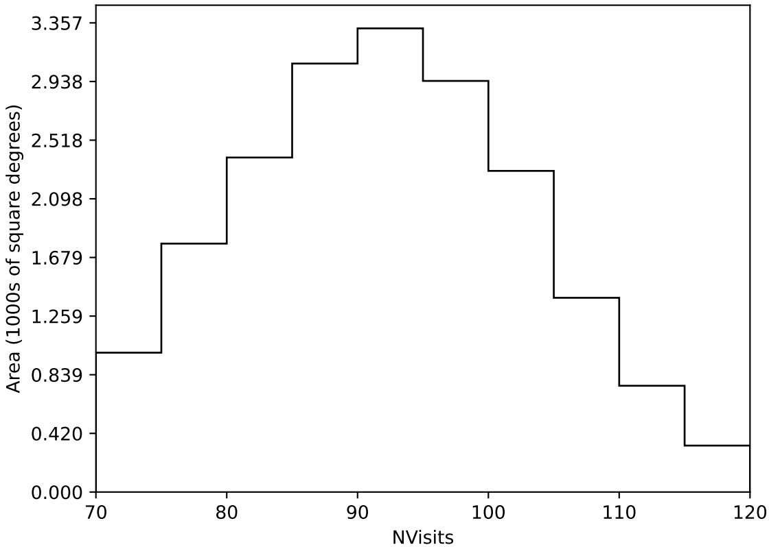
too_elab_2yr_r32_d2_ugrizy_v3.4_10yrs Yr 1 all bands: NVisits
