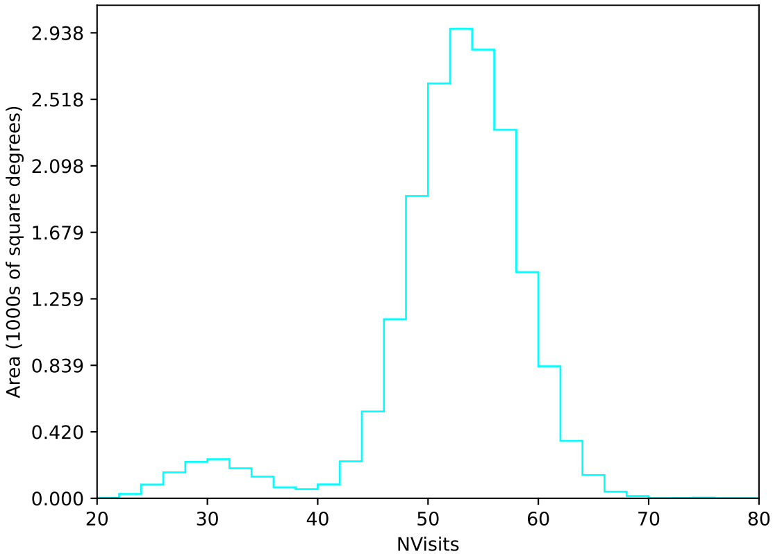
too_elab_2yr_r32_d2_ugrizy_v3.4_10yrs WFD u band: NVisits
