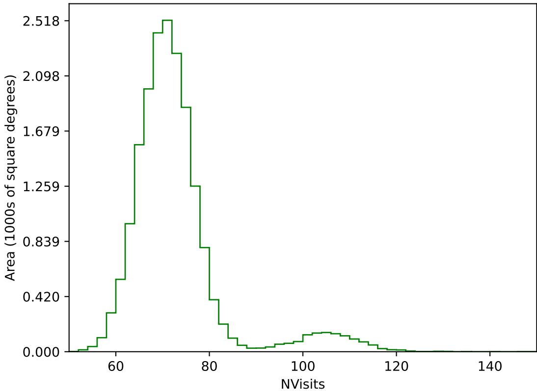
too_elab_2yr_r32_d2_ugrizy_v3.4_10yrs WFD g band: NVisits
