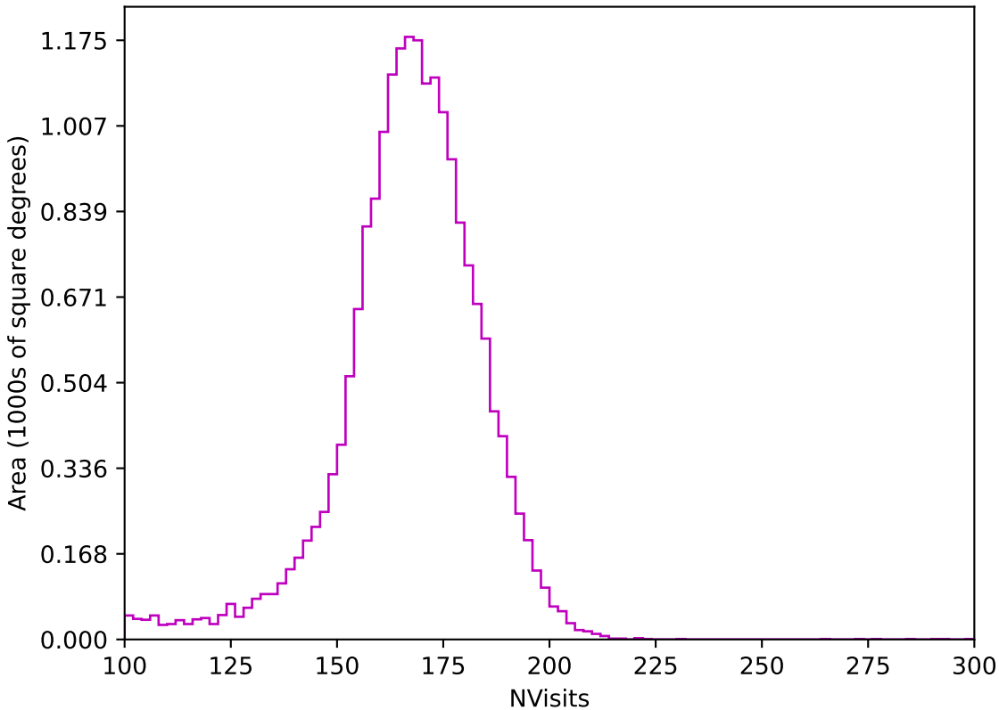
too_elab_2yr_r32_d2_ugrizy_v3.4_10yrs All sky z band: NVisits
