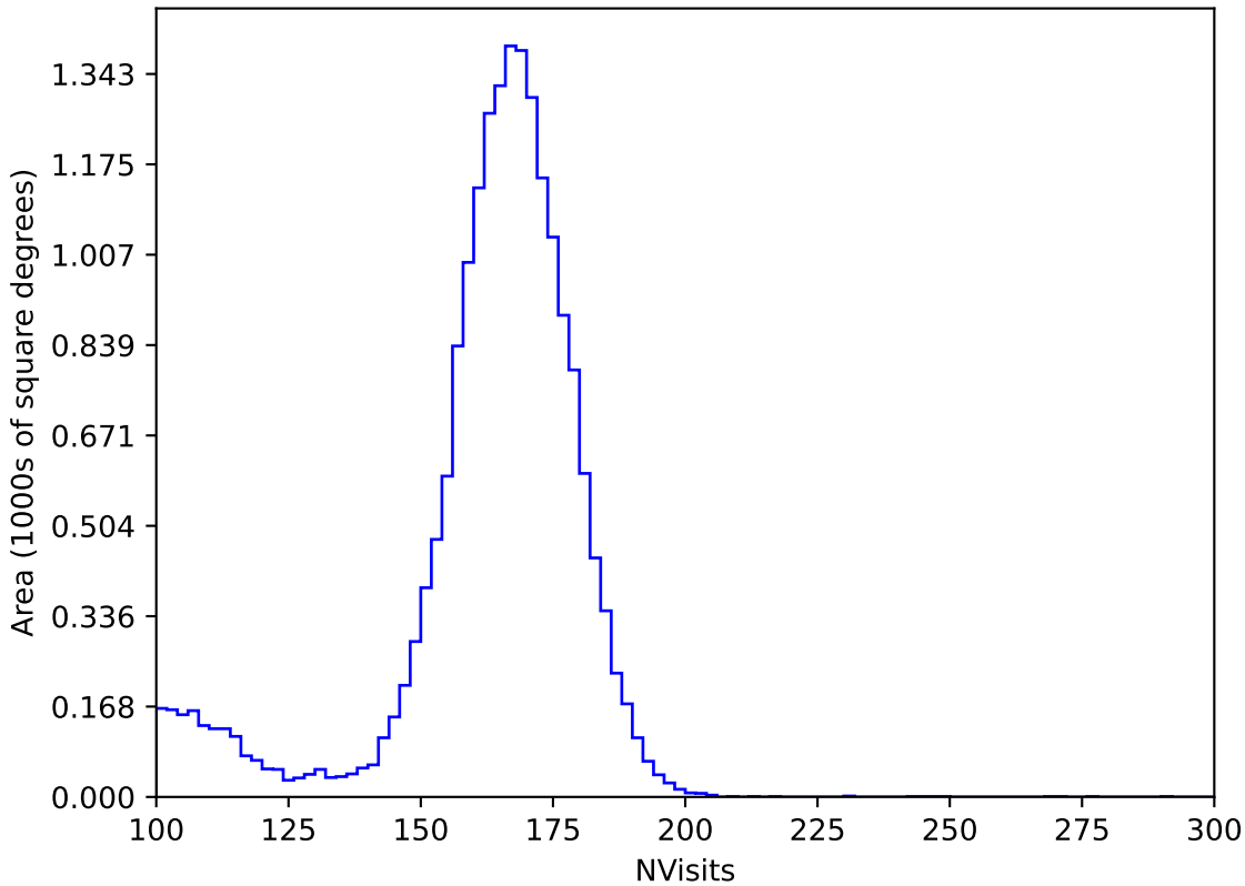
too_elab_2yr_r32_d2_ugrizy_v3.4_10yrs All sky y band: NVisits
