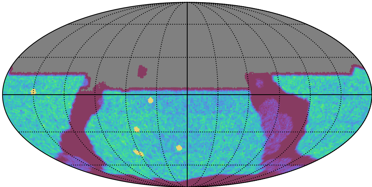
too_elab_2yr_r32_d2_ugrizy_v3.4_10yrs All sky u band: NVisits
