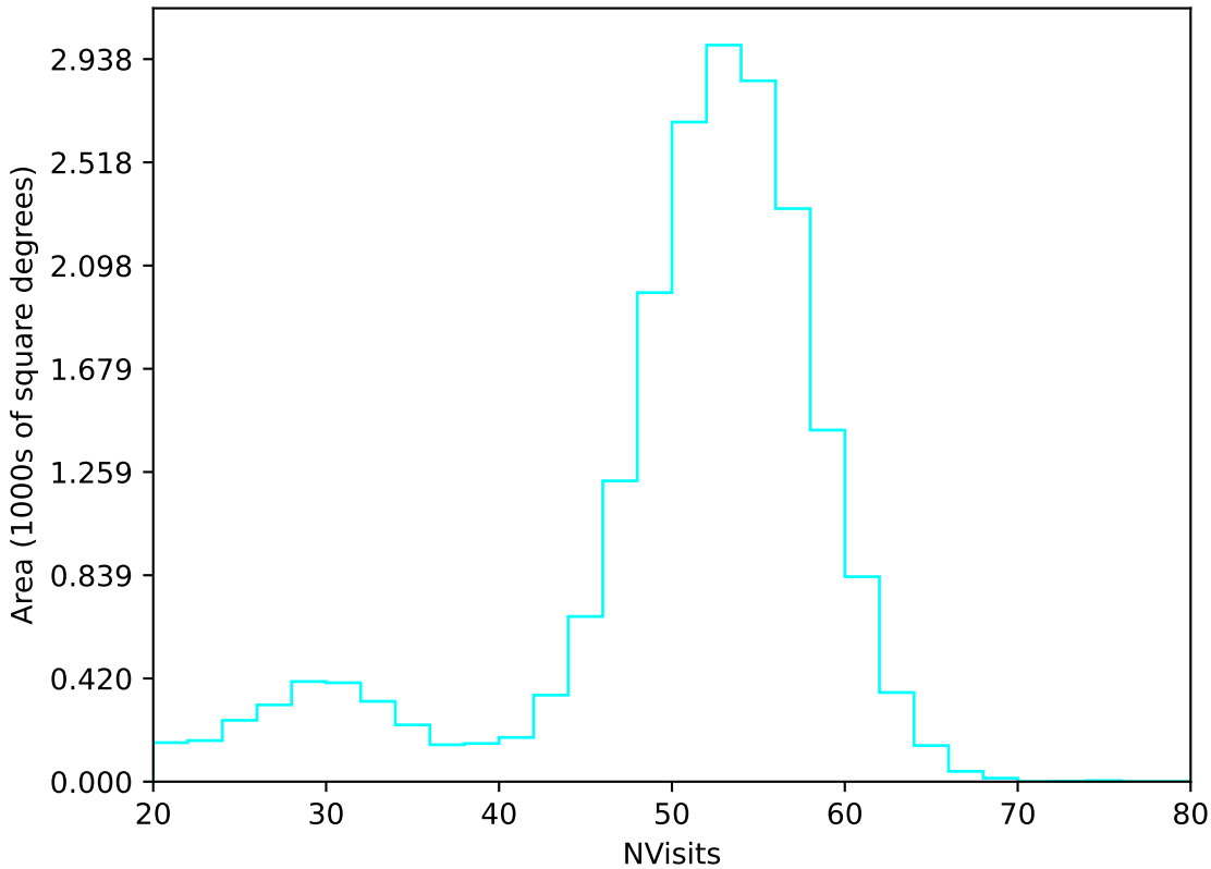
too_elab_2yr_r32_d2_ugrizy_v3.4_10yrs All sky u band: NVisits
