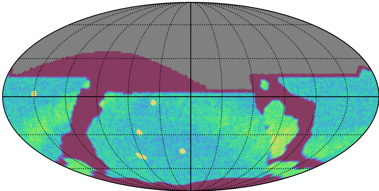
too_elab_2yr_r32_d2_ugrizy_v3.4_10yrs All sky r band: NVisits
