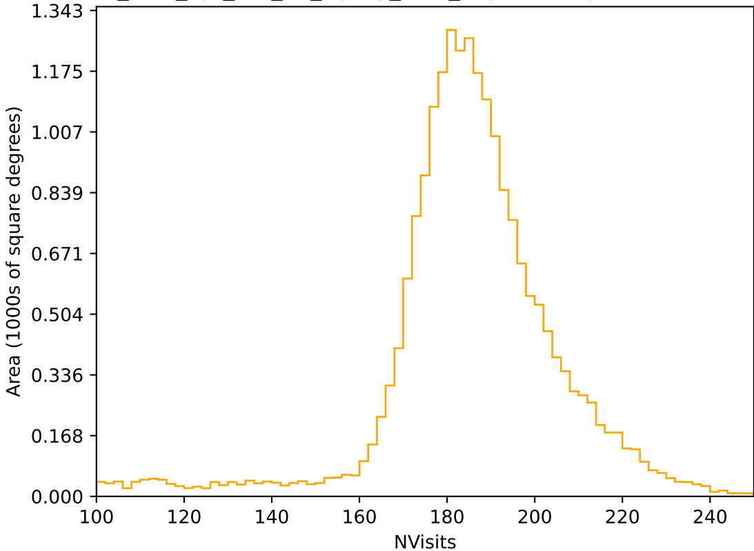
too_elab_2yr_r32_d2_ugrizy_v3.4_10yrs All sky r band: NVisits
