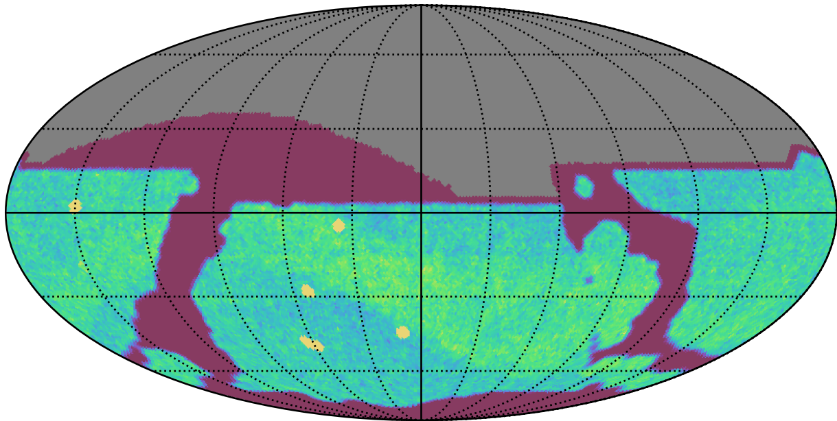
too_elab_2yr_r32_d2_ugrizy_v3.4_10yrs All sky i band: NVisits
