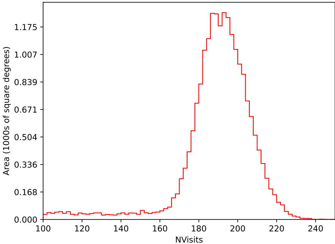
too_elab_2yr_r32_d2_ugrizy_v3.4_10yrs All sky i band: NVisits
