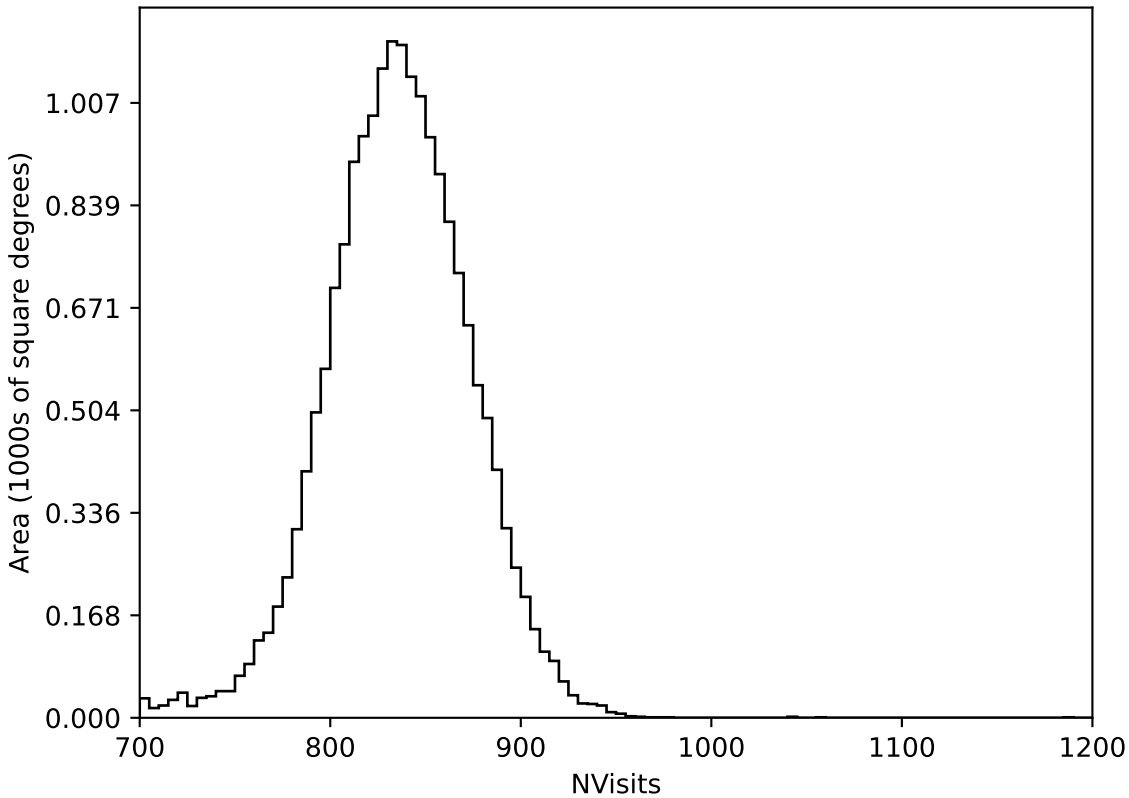
too_elab_2yr_r32_d2_ugrizy_v3.4_10yrs All sky all bands: NVisits
