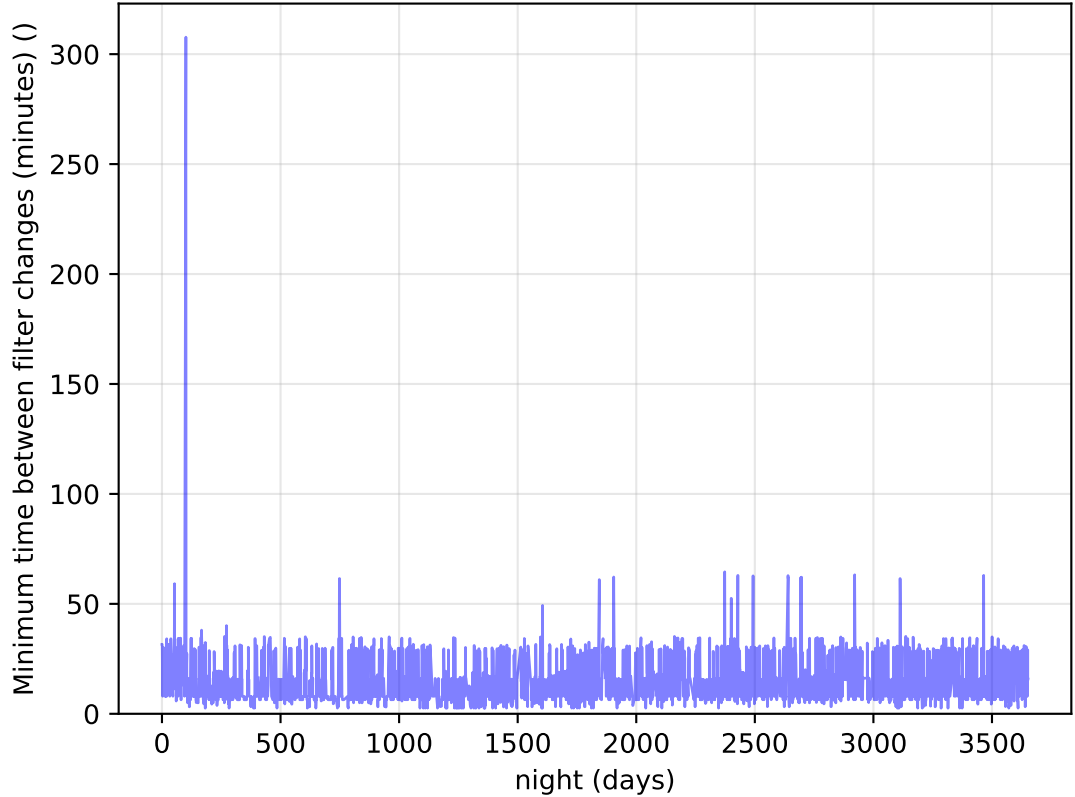
too_elab_2yr_r32_d2_ugrizy_v3.4_10yrs Per Night: Minimum time between filter changes (minutes)
