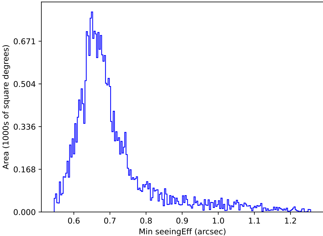
too_elab_2yr_r32_d2_ugrizy_v3.4_10yrs Yr 1 i band: Min seeingEff
