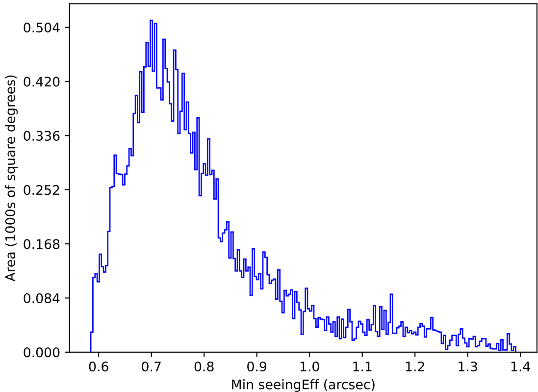
too_elab_2yr_r32_d2_ugrizy_v3.4_10yrs Yr 1 g band: Min seeingEff
