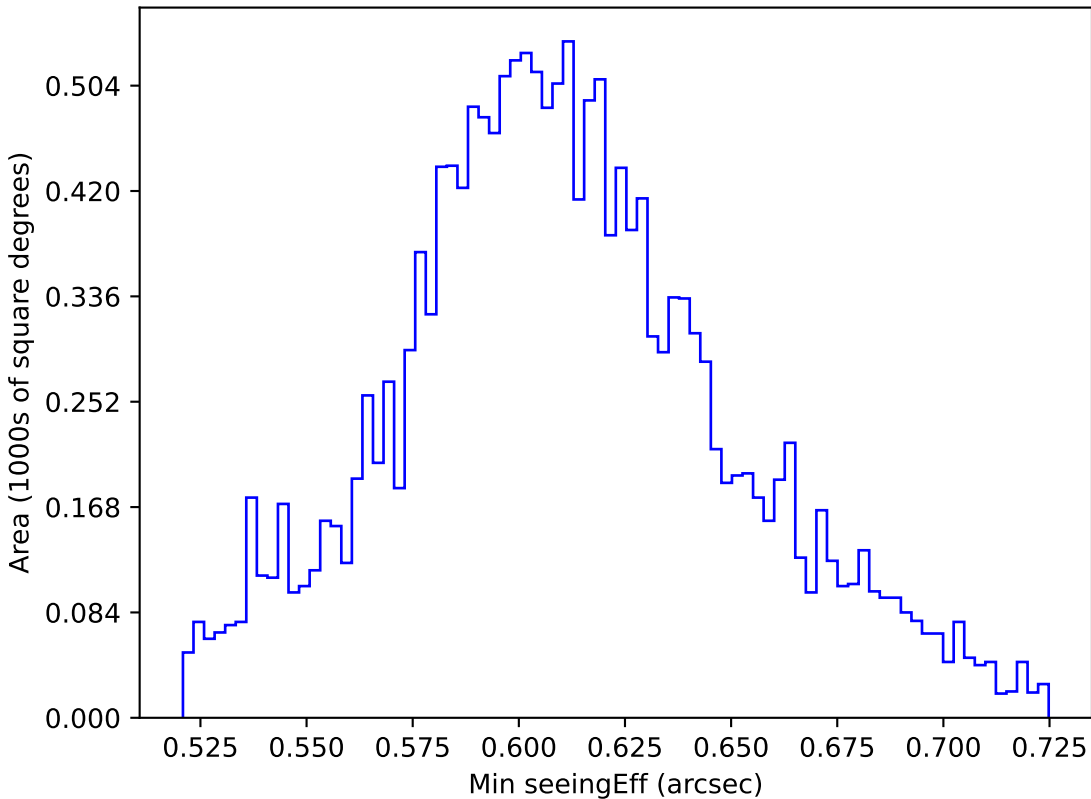
too_elab_2yr_r32_d2_ugrizy_v3.4_10yrs WFD z band: Min seeingEff
