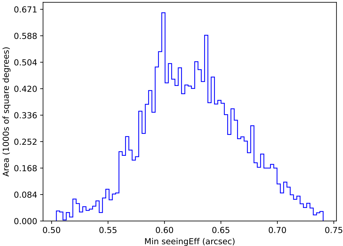
too_elab_2yr_r32_d2_ugrizy_v3.4_10yrs WFD y band: Min seeingEff
