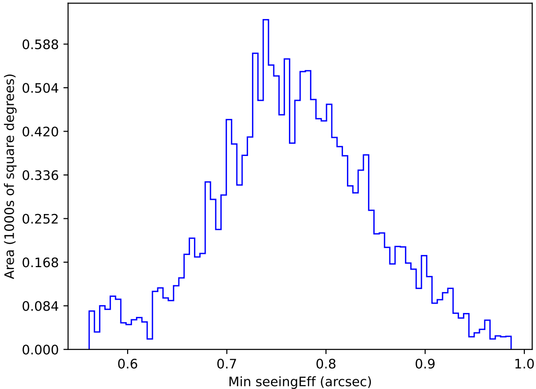
too_elab_2yr_r32_d2_ugrizy_v3.4_10yrs WFD u band: Min seeingEff
