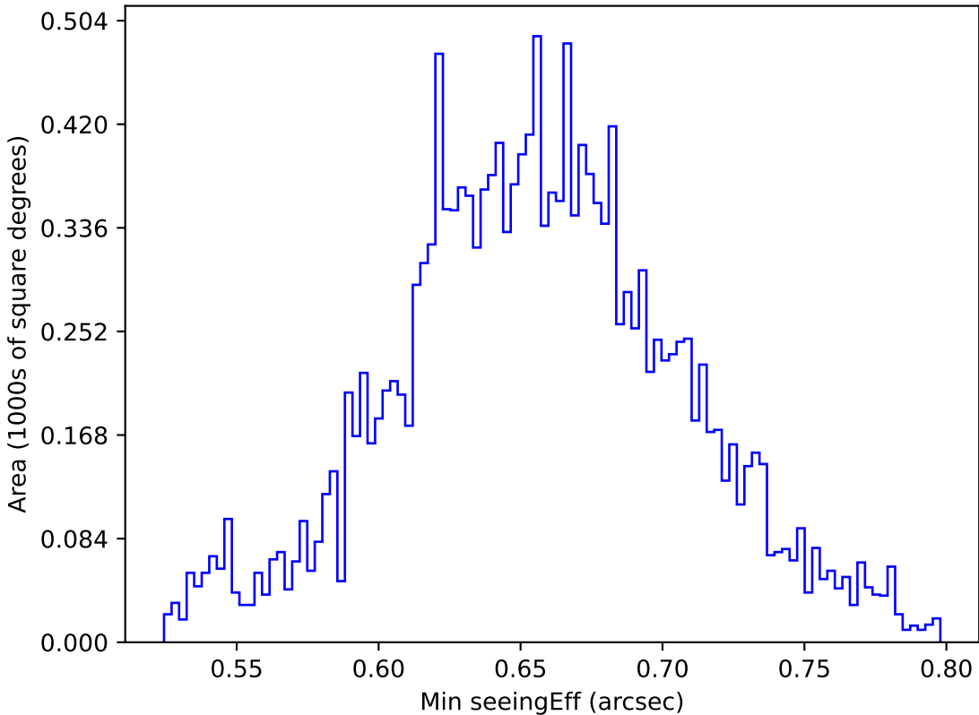
too_elab_2yr_r32_d2_ugrizy_v3.4_10yrs WFD g band: Min seeingEff
