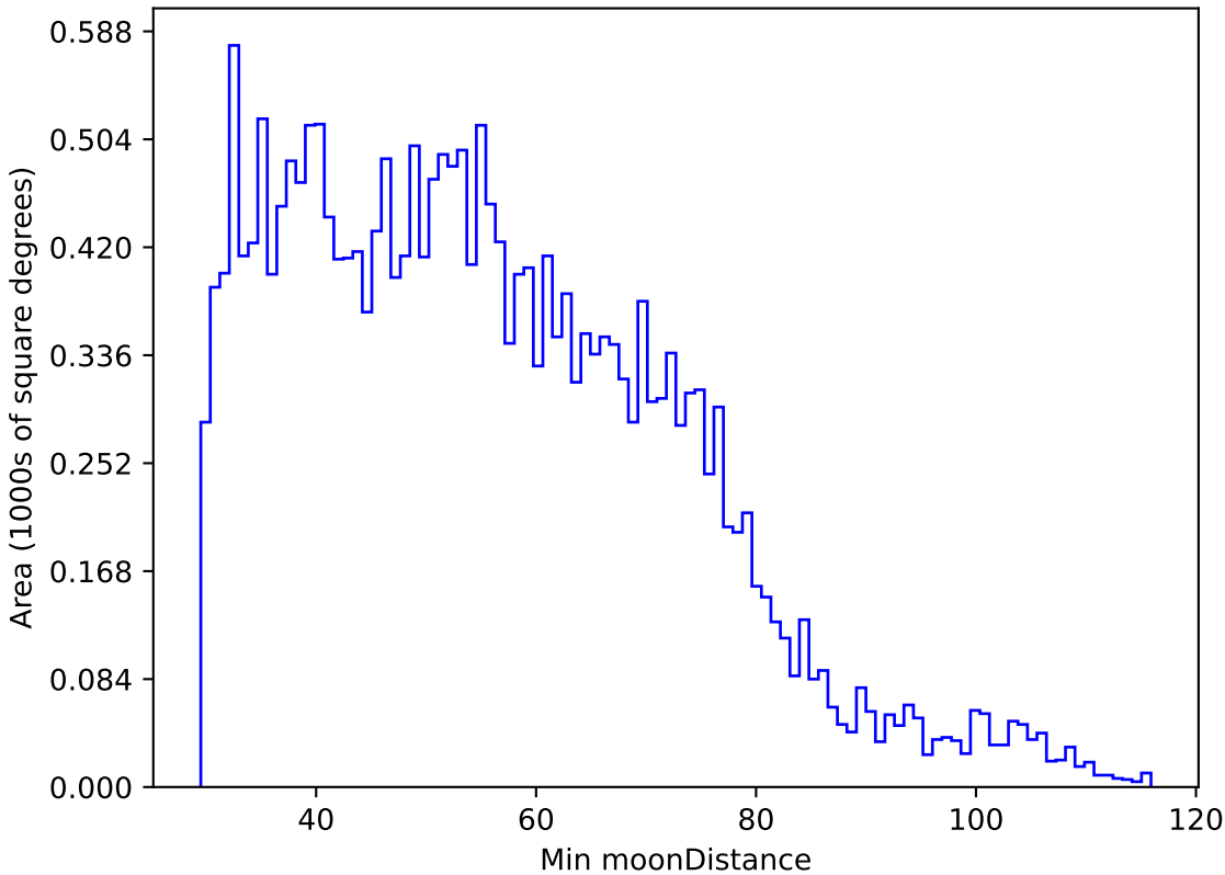
too_elab_2yr_r32_d2_ugrizy_v3.4_10yrs All sky u band: Min moonDistance
