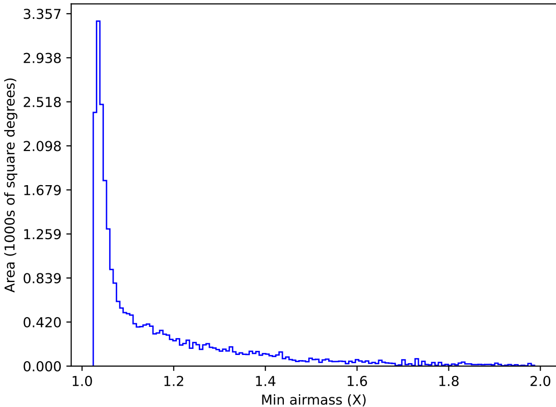
too_elab_2yr_r32_d2_ugrizy_v3.4_10yrs Yr 1 i band: Min airmass
