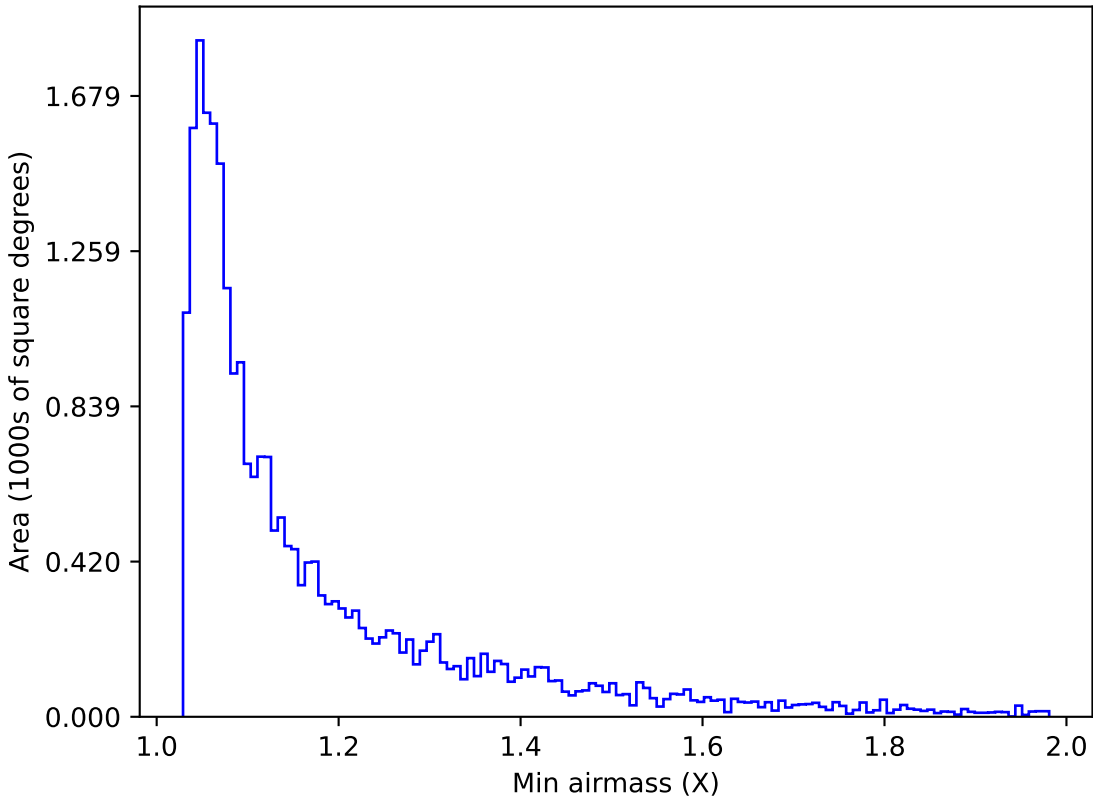
too_elab_2yr_r32_d2_ugrizy_v3.4_10yrs Yr 1 g band: Min airmass
