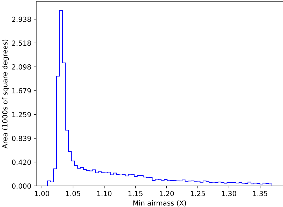
too_elab_2yr_r32_d2_ugrizy_v3.4_10yrs WFD y band: Min airmass
