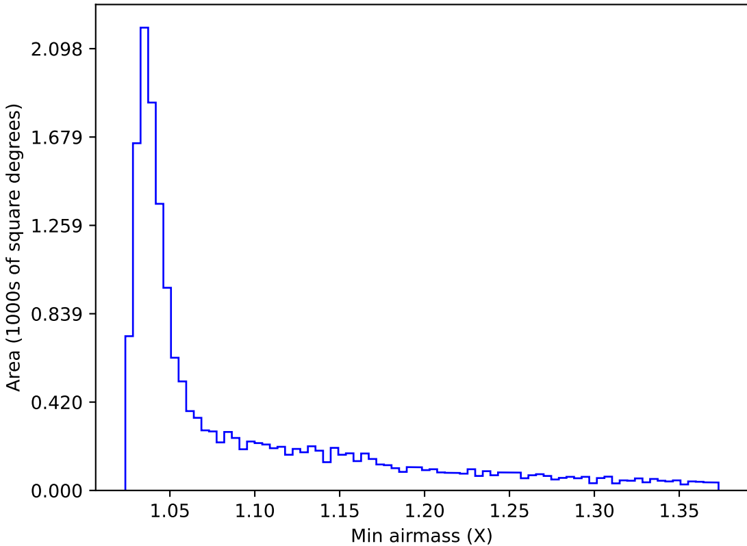
too_elab_2yr_r32_d2_ugrizy_v3.4_10yrs WFD u band: Min airmass
