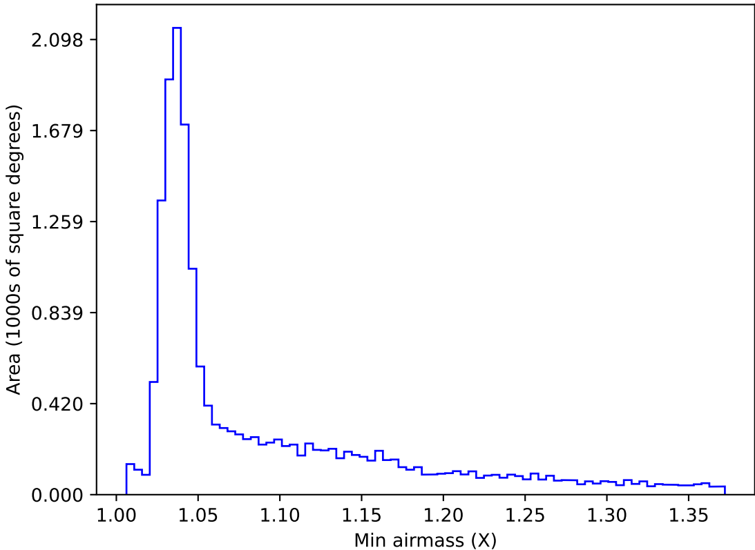
too_elab_2yr_r32_d2_ugrizy_v3.4_10yrs WFD g band: Min airmass
