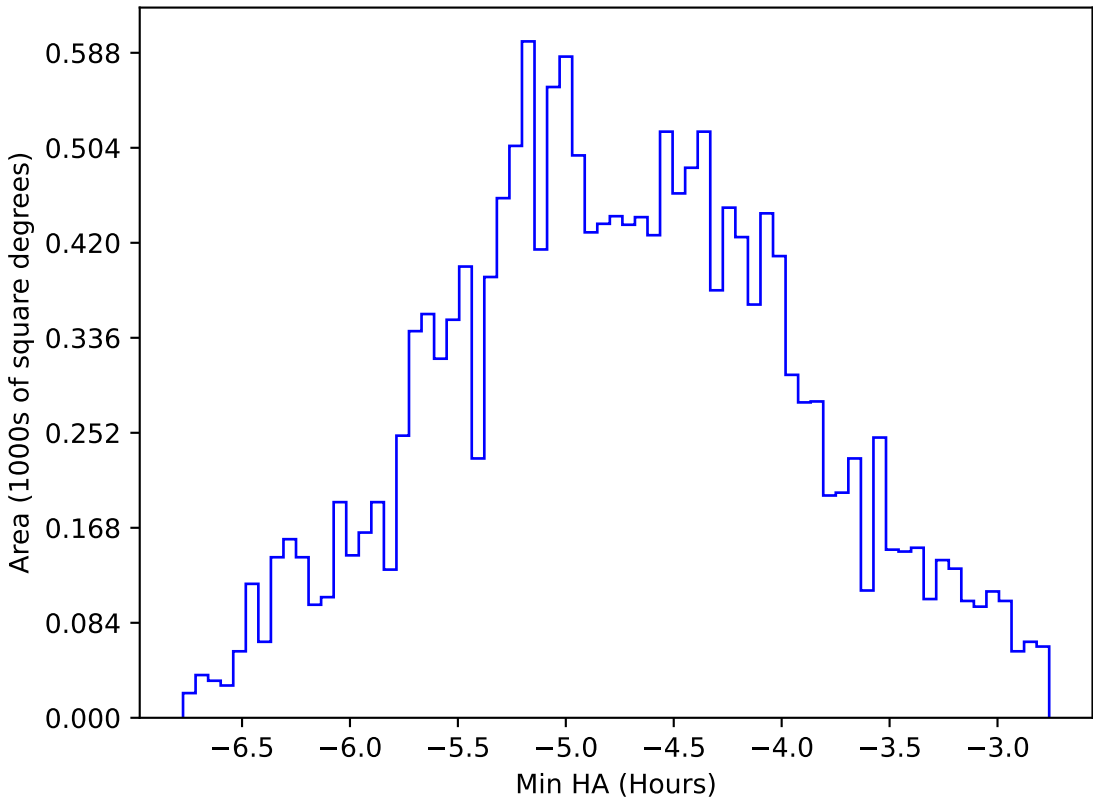
too_elab_2yr_r32_d2_ugrizy_v3.4_10yrs WFD all bands: Min HA
