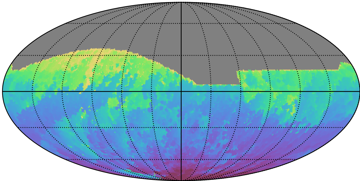
too_elab_2yr_r32_d2_ugrizy_v3.4_10yrs All sky z band: Min HA
