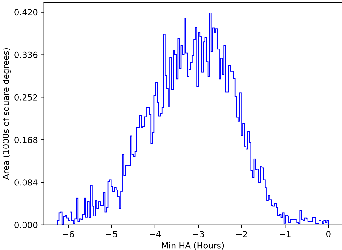
too_elab_2yr_r32_d2_ugrizy_v3.4_10yrs All sky u band: Min HA
