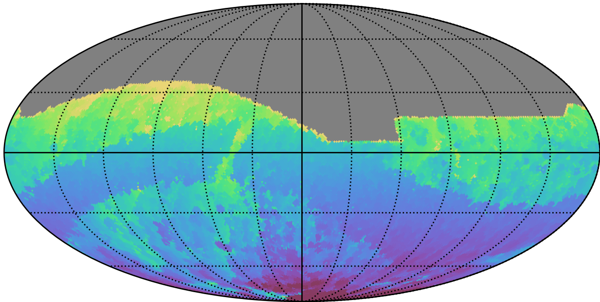
too_elab_2yr_r32_d2_ugrizy_v3.4_10yrs All sky r band: Min HA
