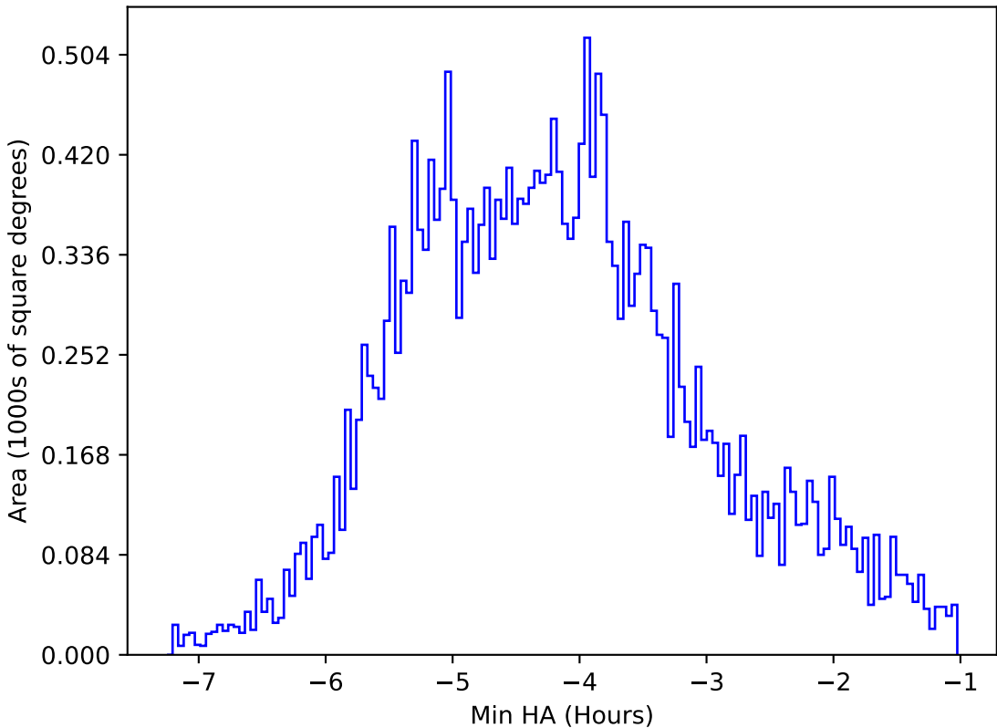
too_elab_2yr_r32_d2_ugrizy_v3.4_10yrs All sky r band: Min HA
