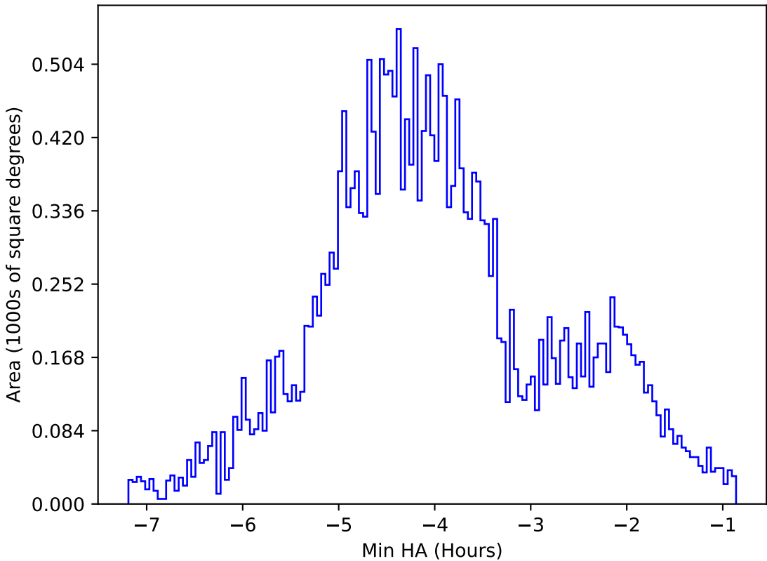
too_elab_2yr_r32_d2_ugrizy_v3.4_10yrs All sky g band: Min HA
