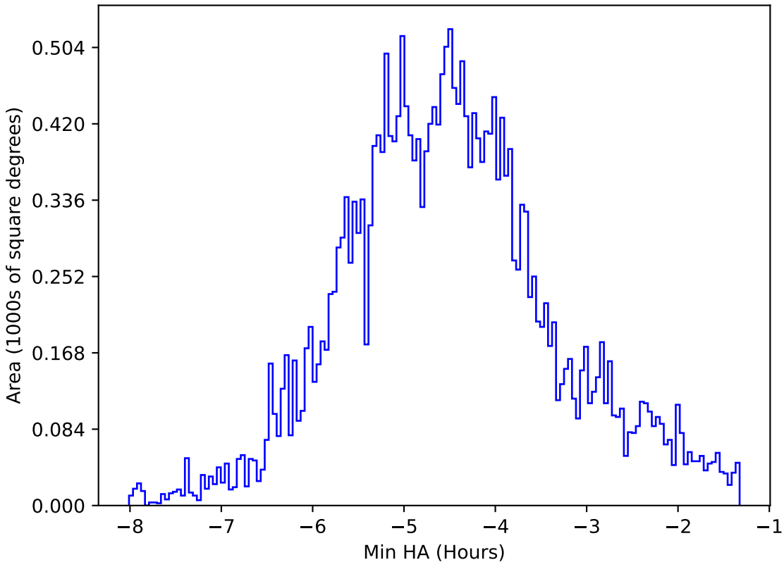
too_elab_2yr_r32_d2_ugrizy_v3.4_10yrs All sky all bands: Min HA
