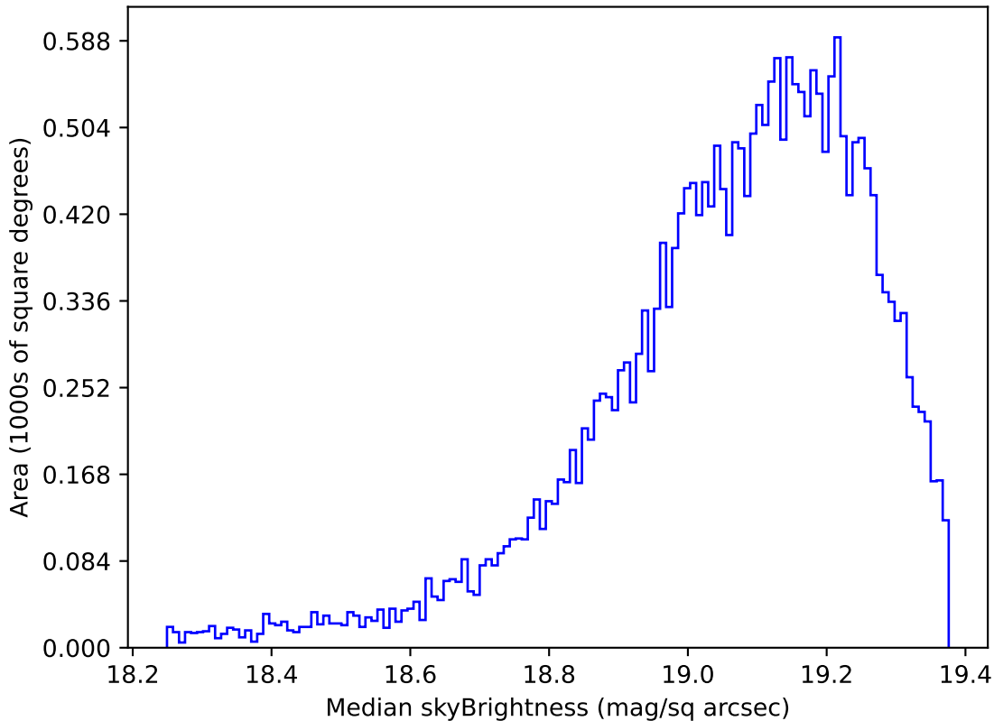
too_elab_2yr_r32_d2_ugrizy_v3.4_10yrs Yr 1 z band: Median skyBrightness
