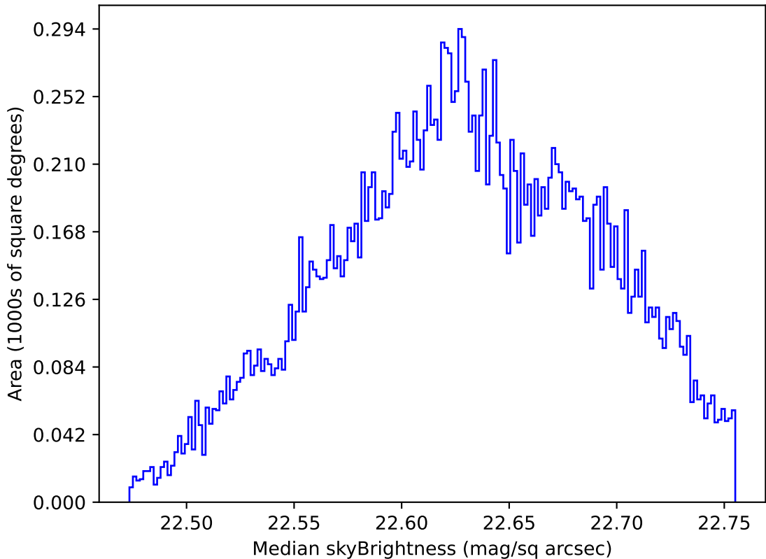
too_elab_2yr_r32_d2_ugrizy_v3.4_10yrs Yr 1 u band: Median skyBrightness
