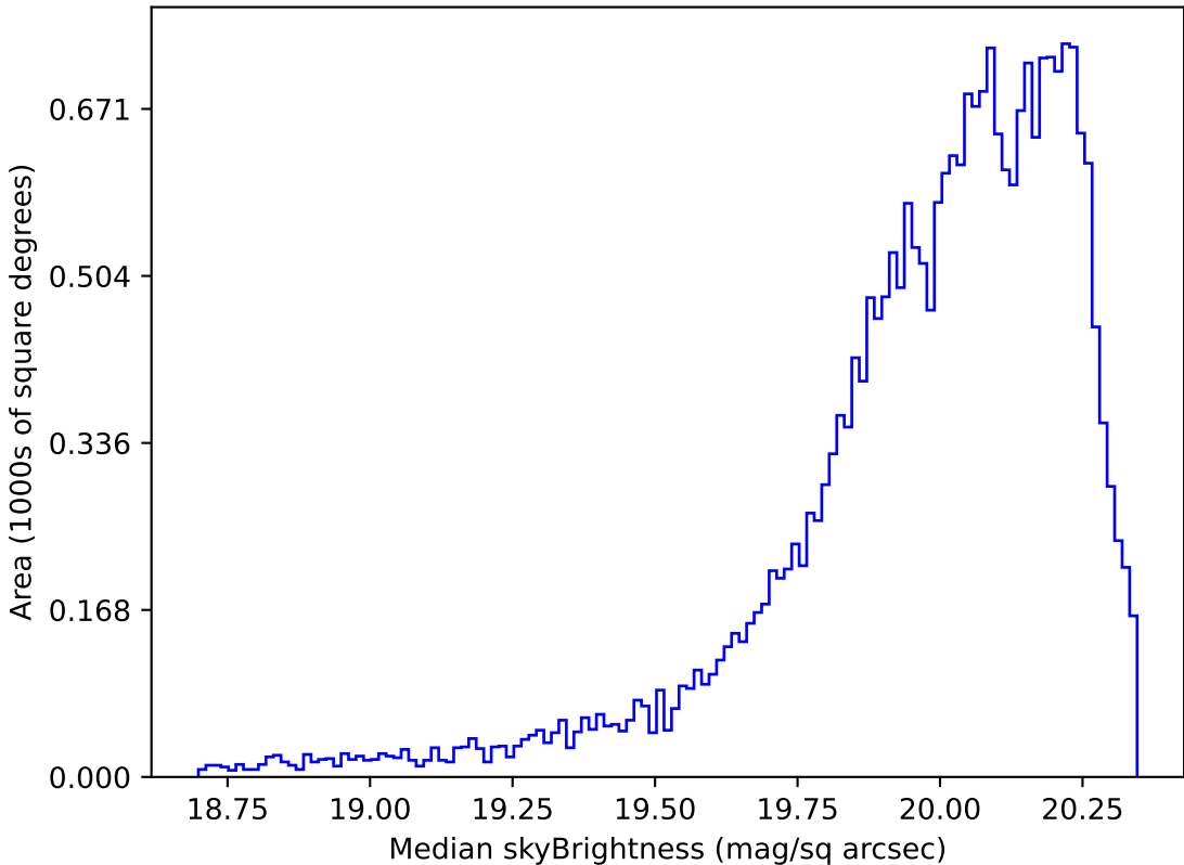
too_elab_2yr_r32_d2_ugrizy_v3.4_10yrs Yr 1 i band: Median skyBrightness
