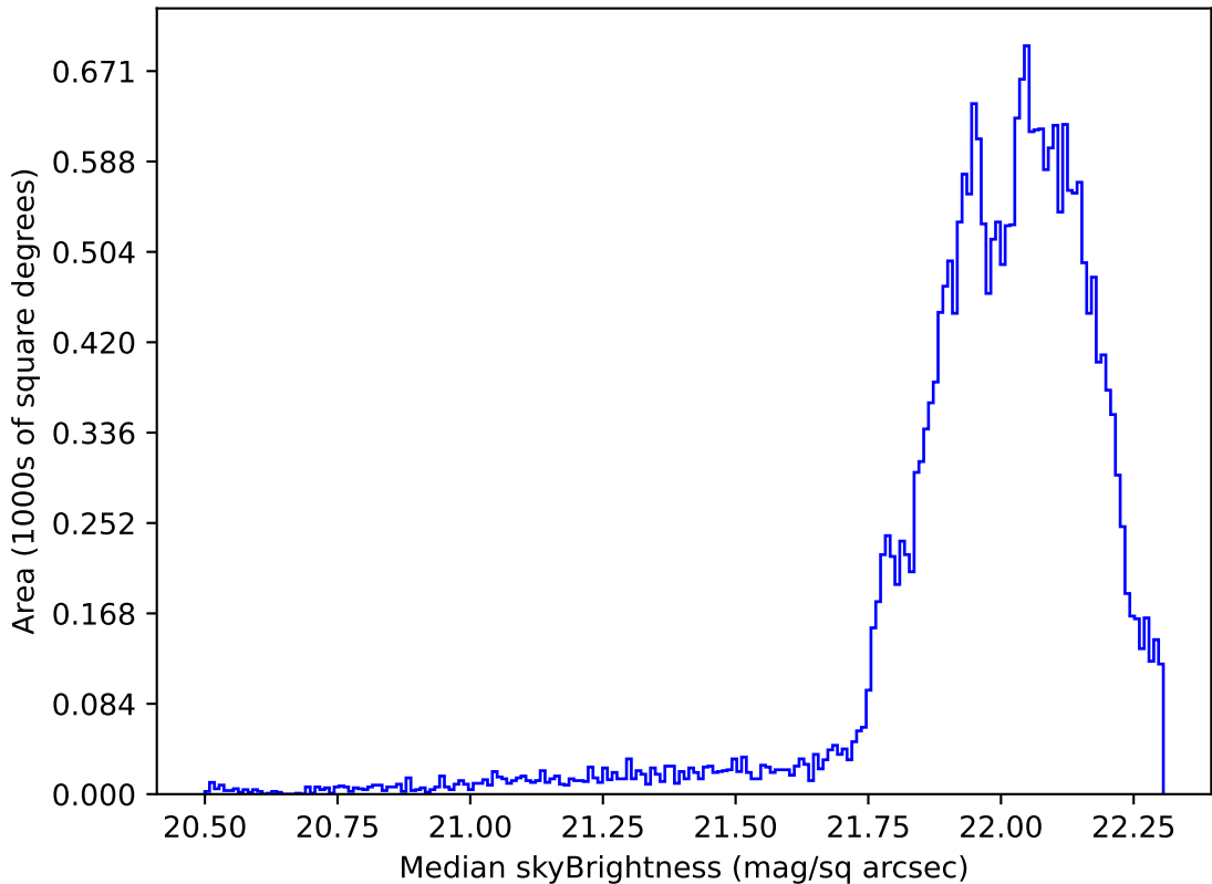
too_elab_2yr_r32_d2_ugrizy_v3.4_10yrs Yr 1 g band: Median skyBrightness
