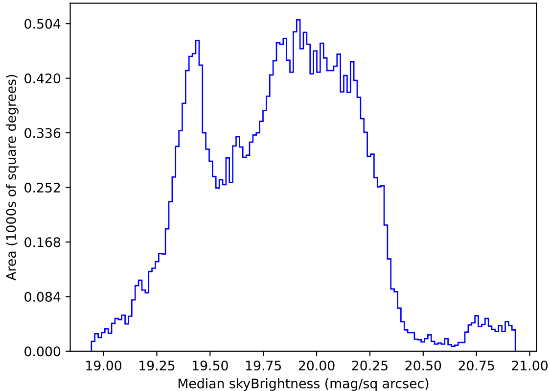
too_elab_2yr_r32_d2_ugrizy_v3.4_10yrs Yr 1 all bands: Median skyBrightness
