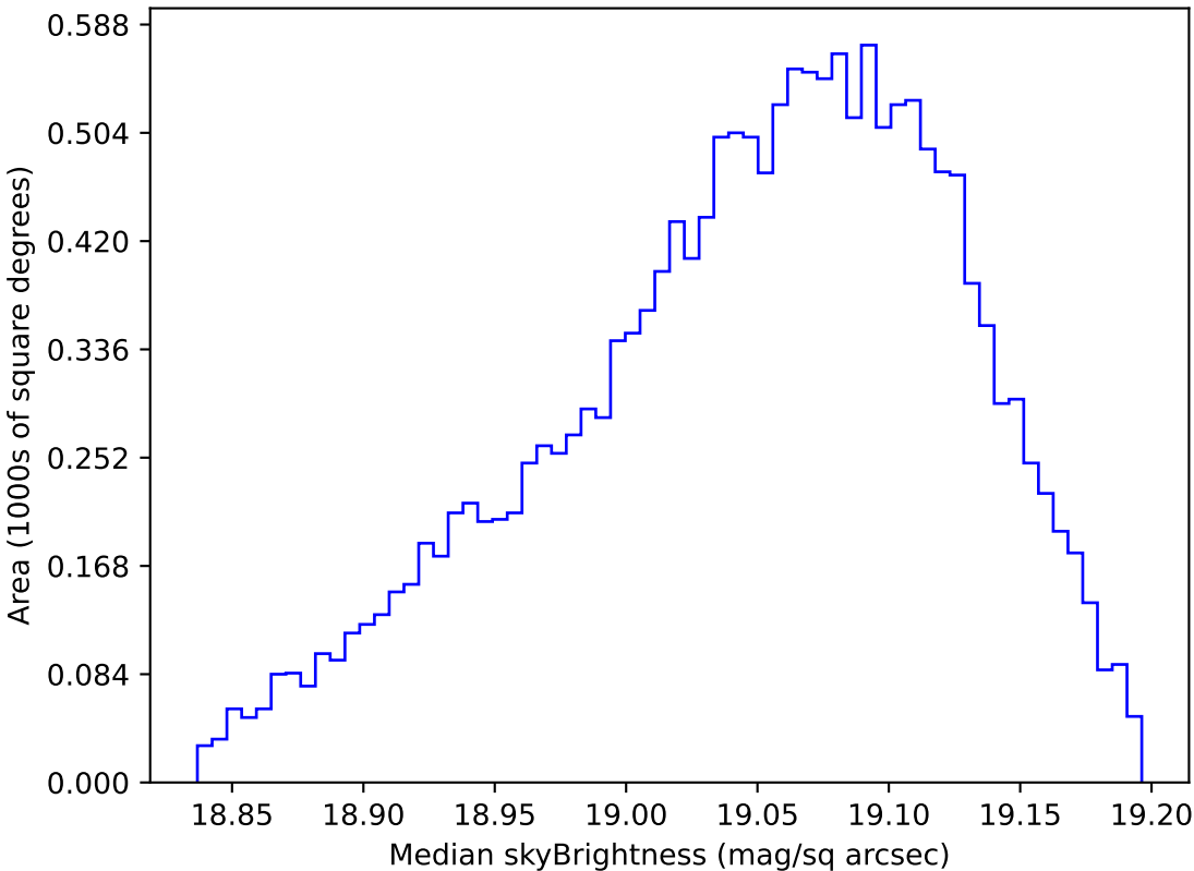
too_elab_2yr_r32_d2_ugrizy_v3.4_10yrs WFD z band: Median skyBrightness
