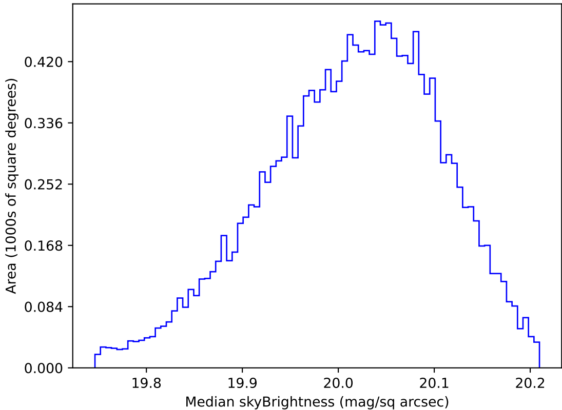
too_elab_2yr_r32_d2_ugrizy_v3.4_10yrs WFD i band: Median skyBrightness
