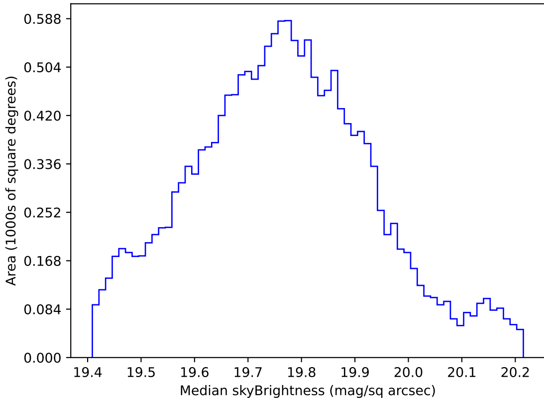
too_elab_2yr_r32_d2_ugrizy_v3.4_10yrs WFD all bands: Median skyBrightness
