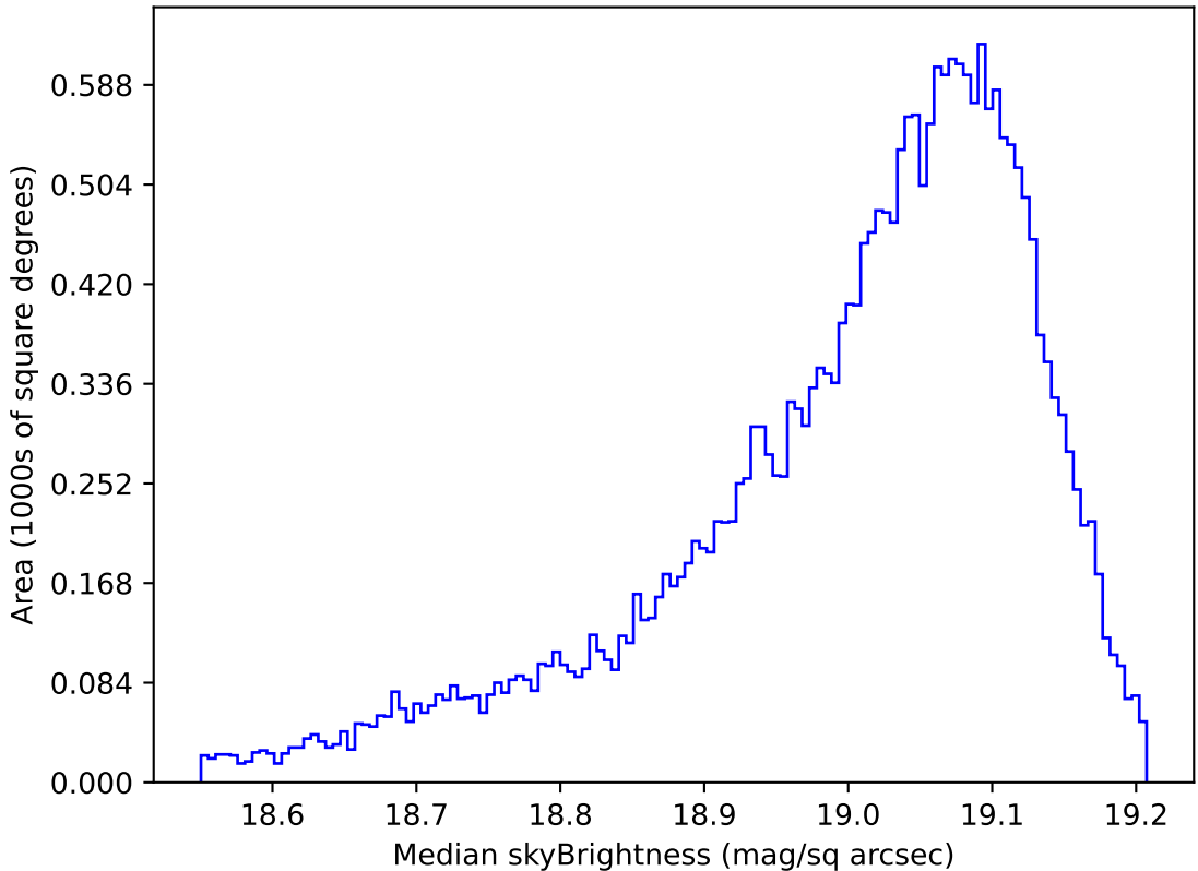
too_elab_2yr_r32_d2_ugrizy_v3.4_10yrs All sky z band: Median skyBrightness
